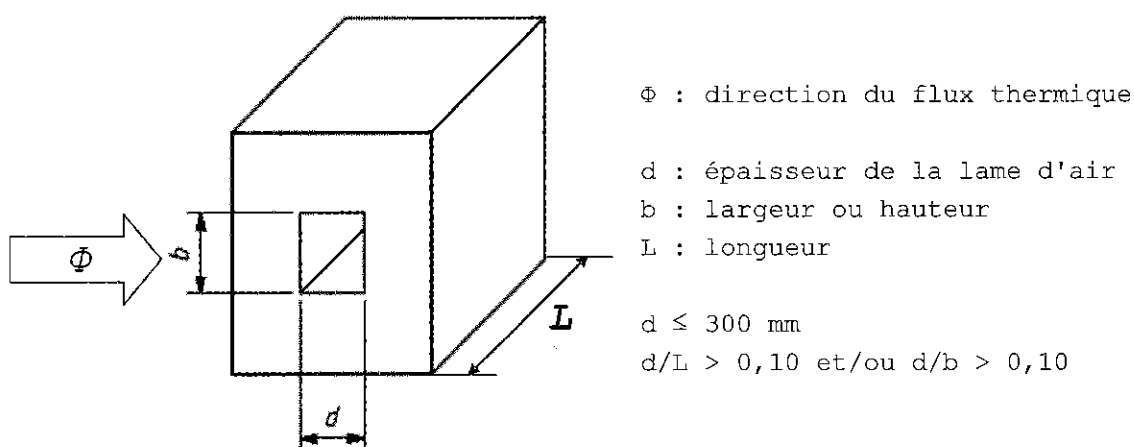
Figure [2] : Creux tubulaires
