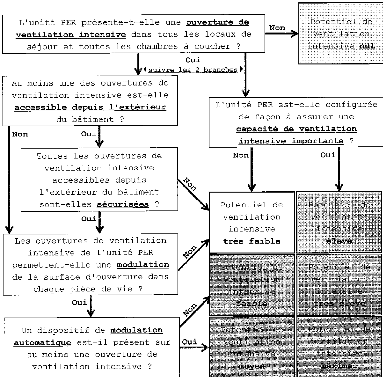
Figure [2] : Potentiel de ventilation intensive
